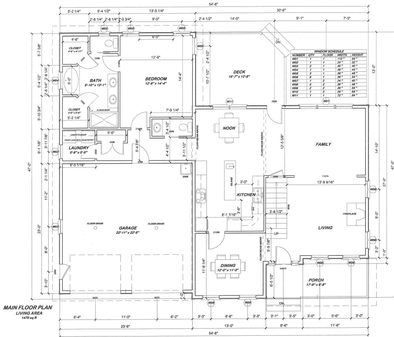
Floor Plan
